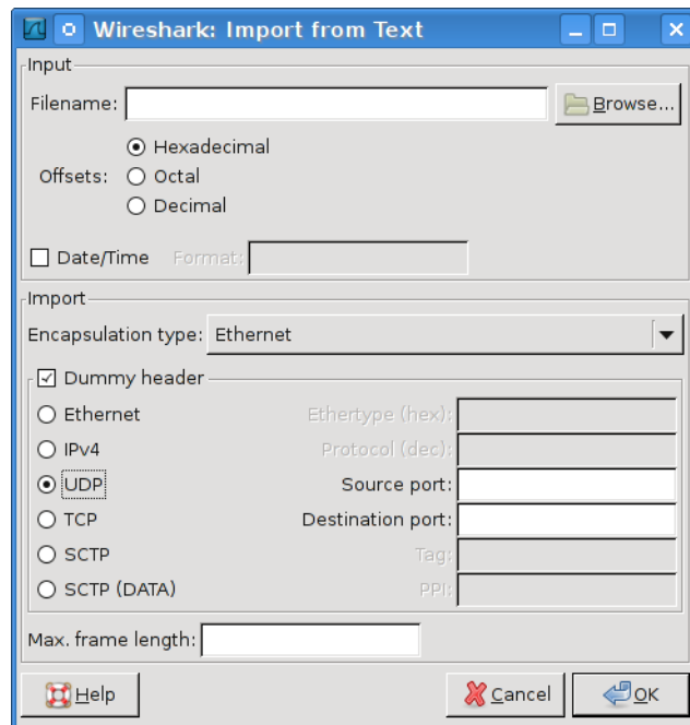
Figure 5.10. The "Import from Hex Dump" dialog
