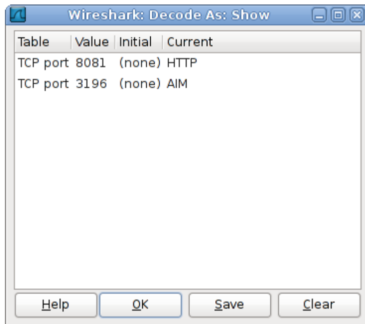
Figure 10.7. The "Decode As: Show" dialog box
